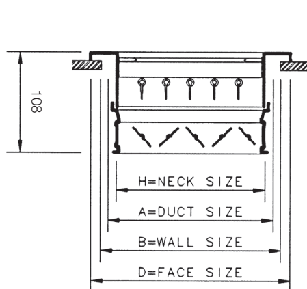
GV/H + G1 Sectional View
