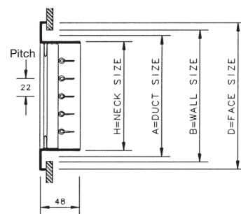
Sectional View
